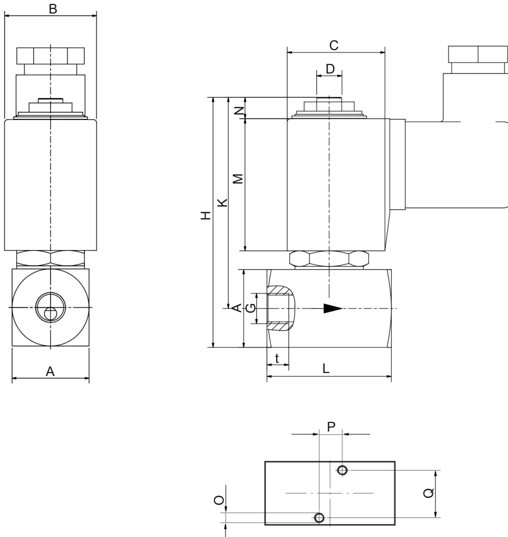
Dimensions, mm
